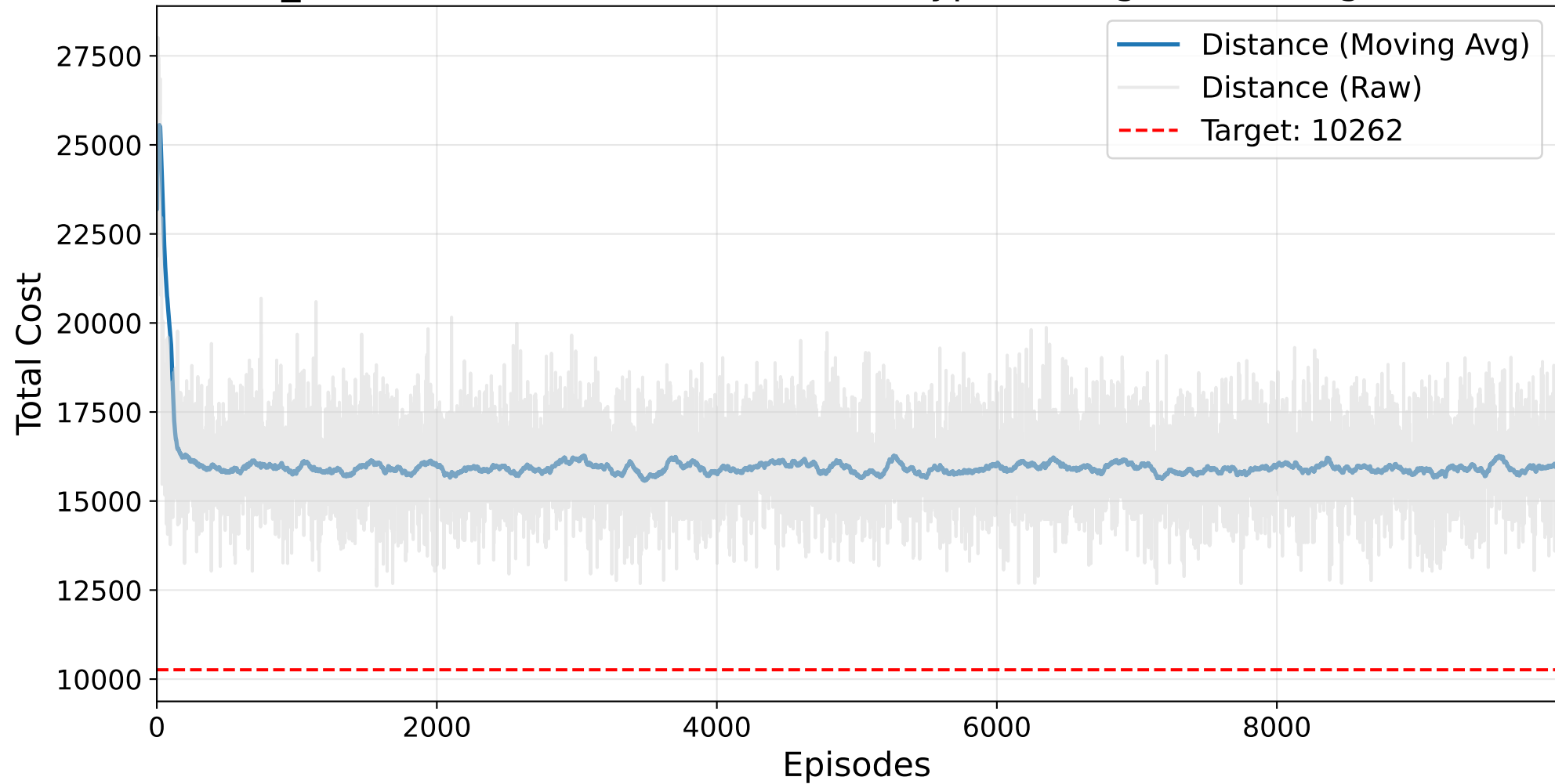
Final NO_BAYESIAN Masked AutoRL-SOP (HyperTuningSK) Training - ft53.3.sop
